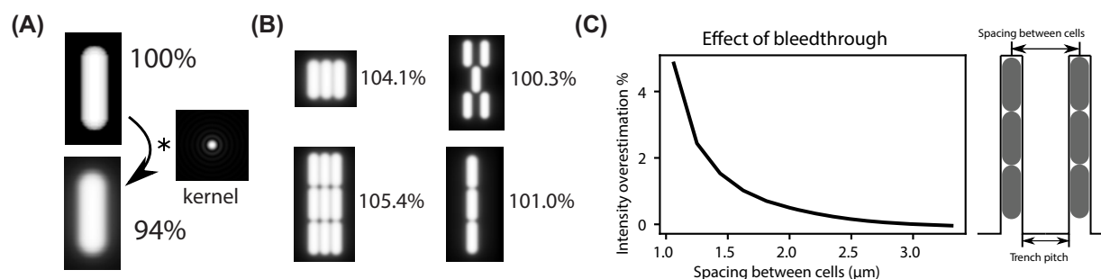
Figure 6. The effects of PSF bleedthrough on intensity measurements
